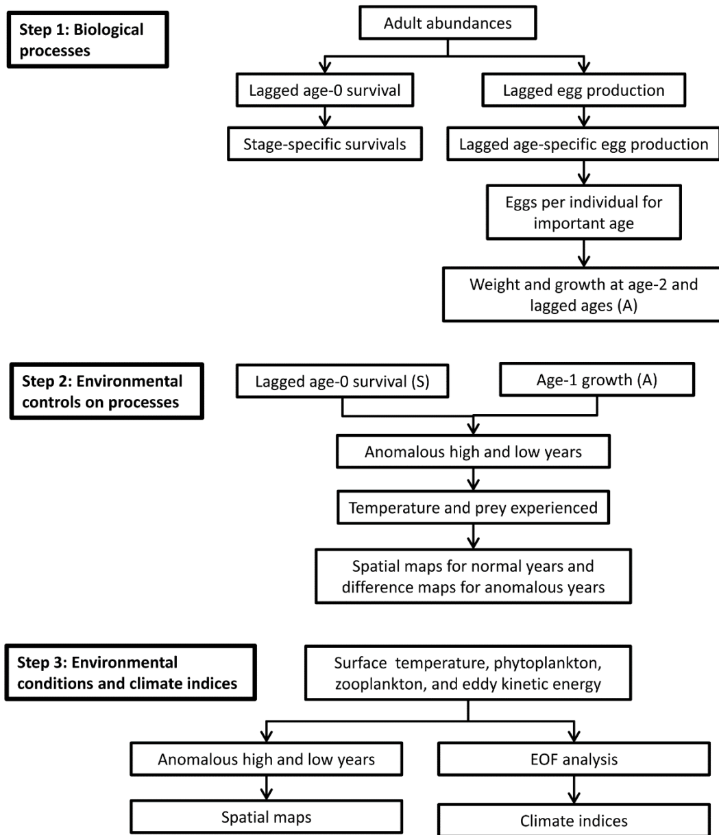
Figure 1: Forensics that outlay multiple processes that may drive recruitment success for anchovies or sardine in the California Current ecosystem (Rose et. al.2015)
