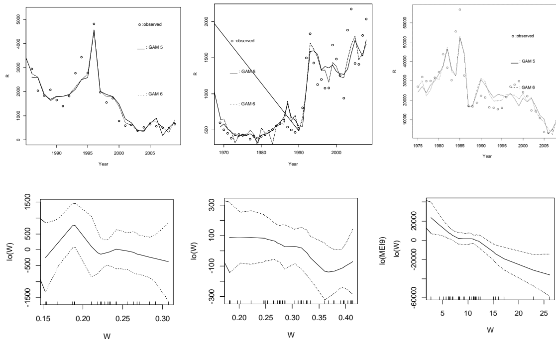
Fig 1. GAM models of recruitment as function of whole numbers of individuals and individual mean weight of the previous year. Upper panel: model fittings; Down panel: Transformed of mean weight recruitment. Left: Hoki; Center: Hake; Right: Jack Mackerel). The transformed of whole numbers of individuals is included in GAM, but not shown in this figure.
